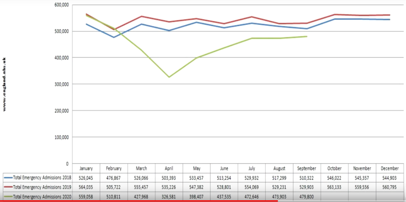
NHS Total Emergency Admissions Jan 2018 - Sept 2020 (Latest Figures)
